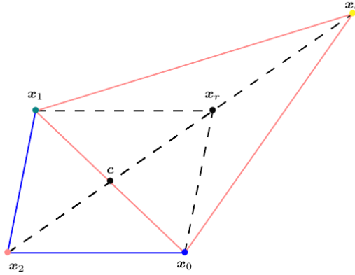
Figure 11.2: The expansion point x_e is computed by moving further away from c .
