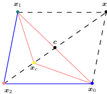
Figure 11.4: The contraction point x_c is computed inside the old simplex.
