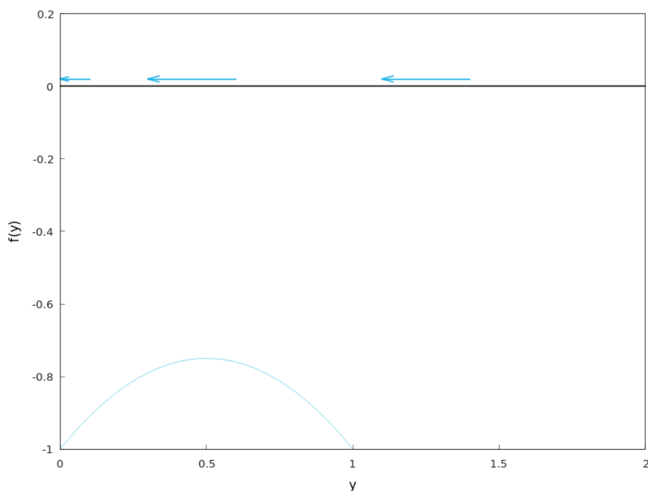
Figure 5.32: The plot for f(y) = (1 - y)y - 1 (Hamzstplot/Examples with Makefile/Plot 2D No Equilibrium Solution for Schaefer Model Variation/main.cpp).
