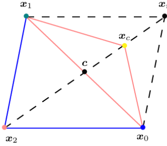
Figure 11.3: The contraction point x_c is computed outside the old simplex.
