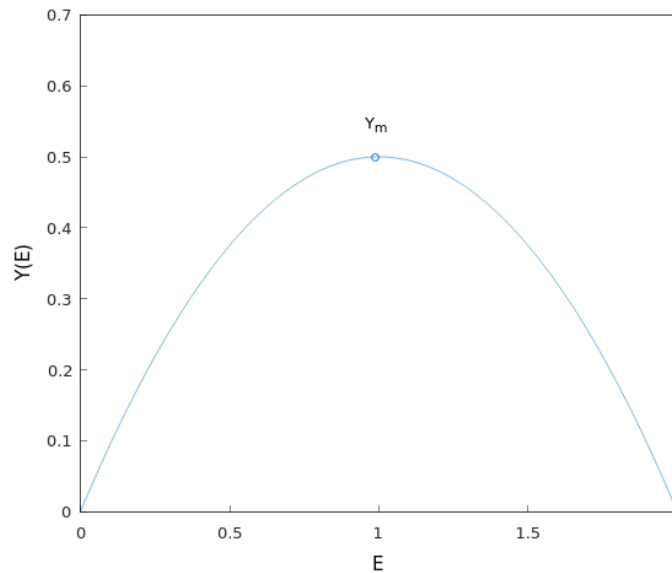
Figure 5.30: The yield-effort curve for Y(E) = EK \left( 1 - \frac{E}{r} \right) with r = 2 and K = 1 (Hamzstplot/Examples with Makefile/Plot 2D Yield-Effort Curve for Schaefer Modell/main.cpp).
