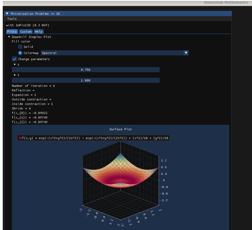
Figure 11.8: The interactive surface plot for f(x,y) = e^{-\frac{x^2+y^2}{2s^2}} - e^{-\frac{x^2+y^2}{2t^2}} + \frac{1}{10}x^2 + \frac{1}{10}y^2 , s = 0.75 , t = 1 with Hamzstlab Mathematics. (Hamzstlab-Mathematics/examples/3D Minimization/main.cpp).
