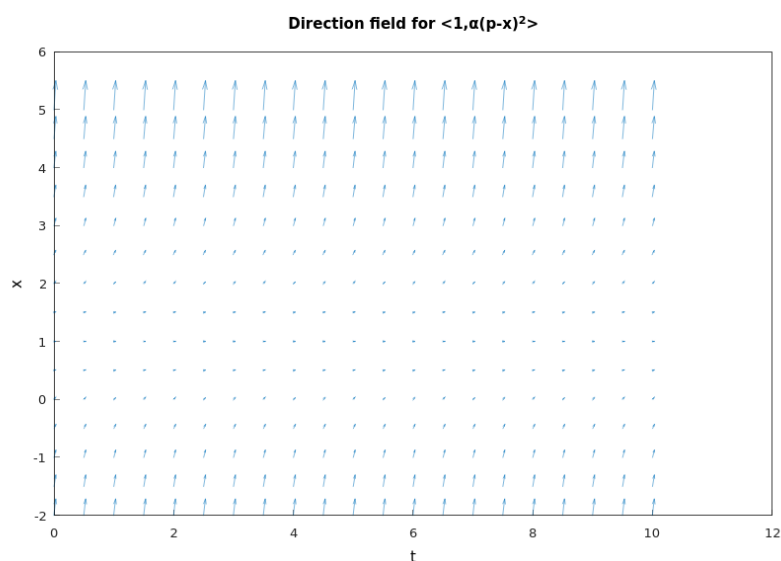
Figure 5.50: The direction field for \langle 1, \alpha(p-x)^2 \rangle with \alpha = 1 and p = 1 (Hamzstplot/Examples with Makefile/Plot Direction Fields for Chemical Reactions Problem 28b/main.cpp).
