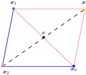
Figure 11.1: x_2 is mirrored in c and creates a reflected point x_r .
