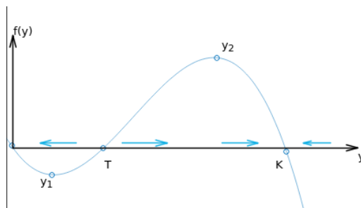
Figure 5.27: The graph of f(y) versus y for logistic growth with a threshold for \frac{dy}{dt} = -r \left(1 - \frac{y}{T}\right) \left(1 - \frac{y}{K}\right) y (Hamzstplot/Examples with Makefile/Plot 2D Equilibrium Solution for Logistic Growth with a Threshold/main.cpp).
