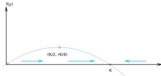
Figure 5.22: The equilibrium solution f(y) = 0 or r(1 - y/K)y = 0 to visualize other solutions of Eq. (4.53) ( Hamzstplot/Examples with Makefile/Plot 2D Equilibrium Solution for Logistic Growth/main.cpp ).
