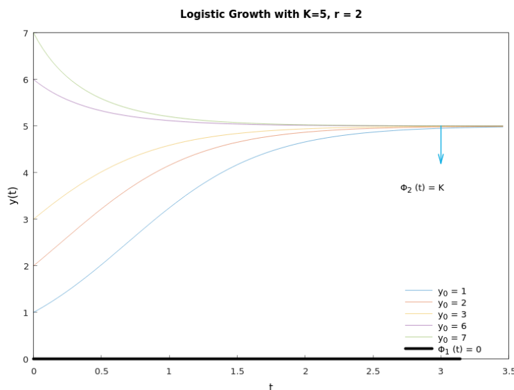
Figure 5.23: The solution curves for y(t) = \frac{y_0 K}{y_0 + (K - y_0)e^{-rt}} to visualize all possible solutions of Eq. (4.53) with different y_0 (Hamzstplot/Examples with Makefile/Plot 2D Solution Curves for Logistic Growth/main.cpp).
