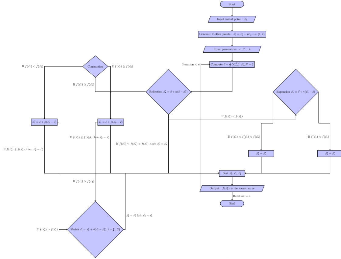
Figure 11.6: The flowchart for downhill simplex algorithm that is used to make the C++ code for computing the solution.
