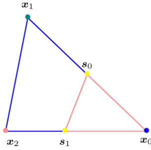
Figure 11.5: Shrink the simplex by moving every point closer to the current best.
